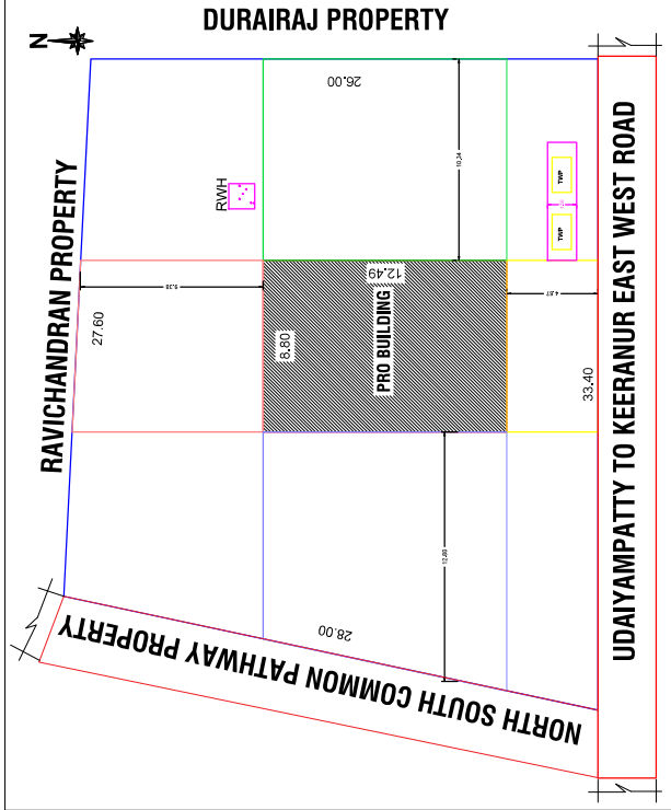
SITE PLAN
