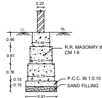
FOOTING DETAIL (NOT TO SCALE)
