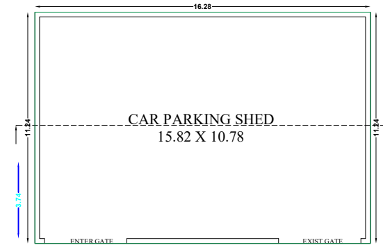
FLOOR - GROUND GROUND FLOOR PLAN
