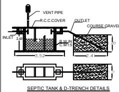
SEPTIC TANK & D-TRENCH DETAILS
