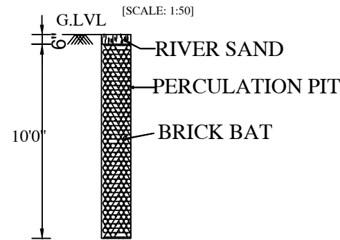
PERCOLATION PIT
