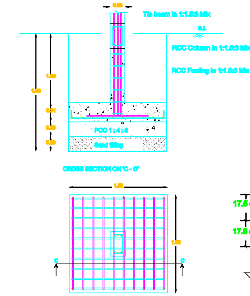
COLOUMN FOUNDATION DETAILS
