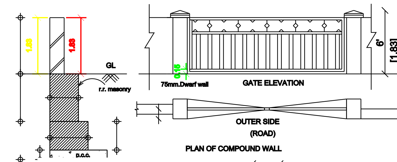
PLAN OF COMPOUND WALL
