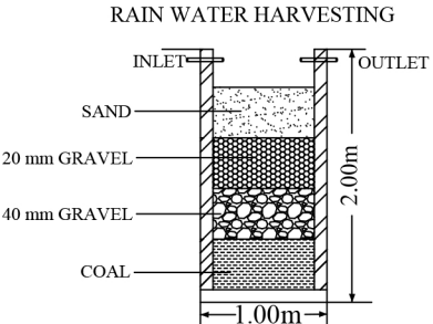
RAIN WATER COLLECTION TANK
