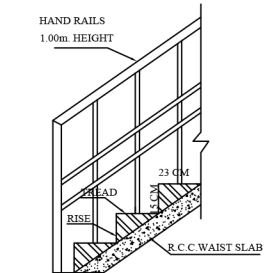
SECTION ON STAIRCASE
