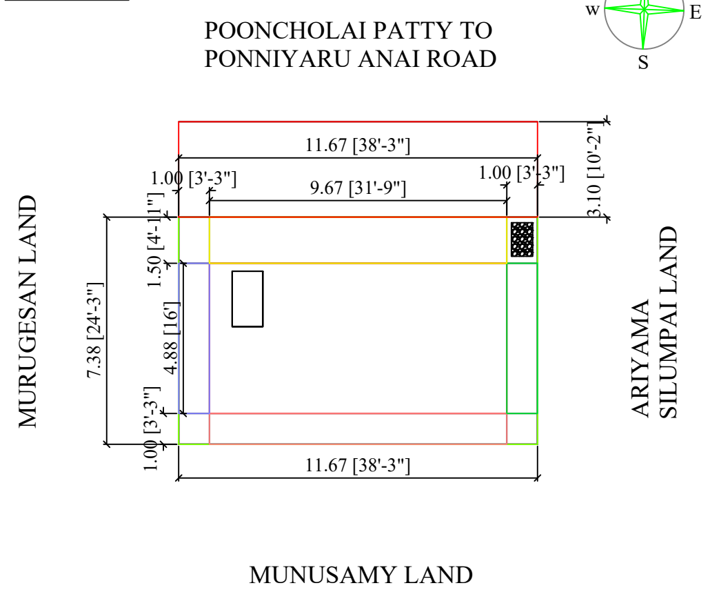
SITE PLAN
