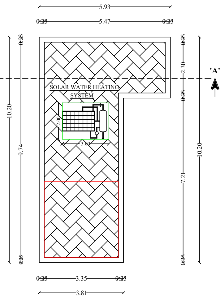
FLOOR - TERRACE
