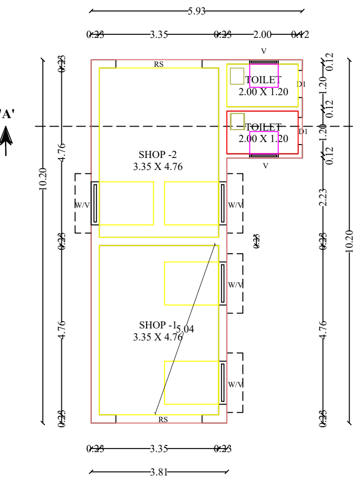
FLOOR - GROUND
