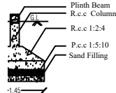
FOOTING DETAILS
