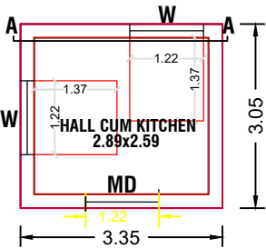
PRO., GROUND FLOOR PLAN
