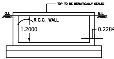
RWH SECTION (SAMPLE) RWHT_CAPACITY_L=2000LTRS
