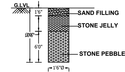
RAIN WATER HARVESTING PIT (NOT TO SCALE)
