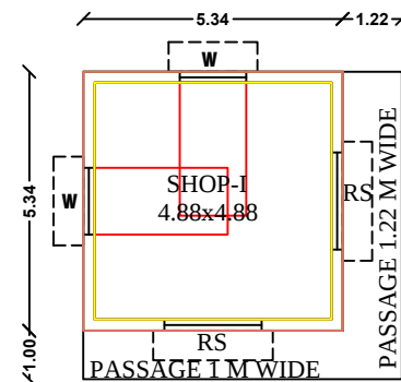
BLOCK IV PROPOSED GROUND FLOOR PLAN
