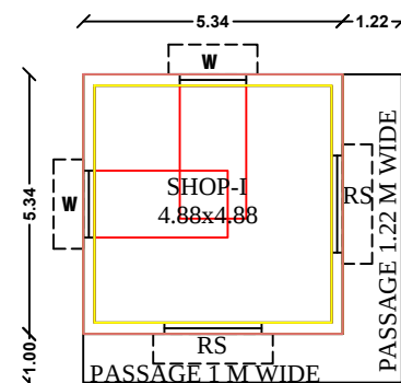
BLOCK III PROPOSED GROUND FLOOR PLAN
