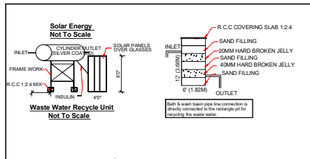
PERCOLATION PIT
