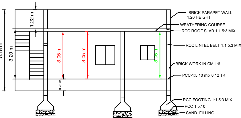
SECTION " AB "
