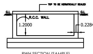
RWH_CAPACITY_L=2000LTRS
