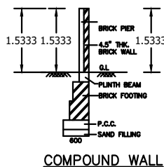
COMPOUND WALL
