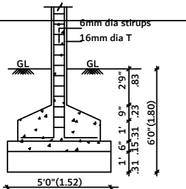
COLUMN FOUNDATION DETAIL
