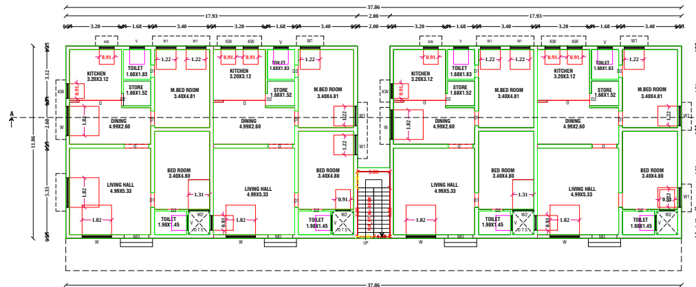
FLOOR - GROUND PRO. GROUND FLOOR PLAN
