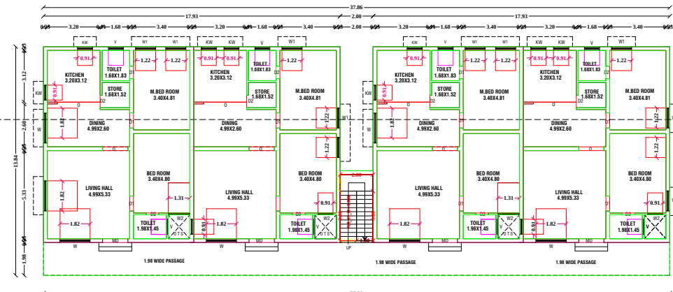
FLOOR - FIRST PRO. FIRST FLOOR PLAN
