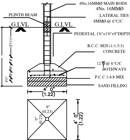
FOUNDATION DETAIL
