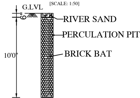
PERCOLATION PIT
