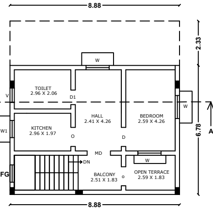
PROPOSED SECOND FLOOR - PLAN
