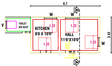
GROUND FLOOR
