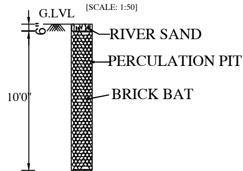
PERCOLATION PIT
