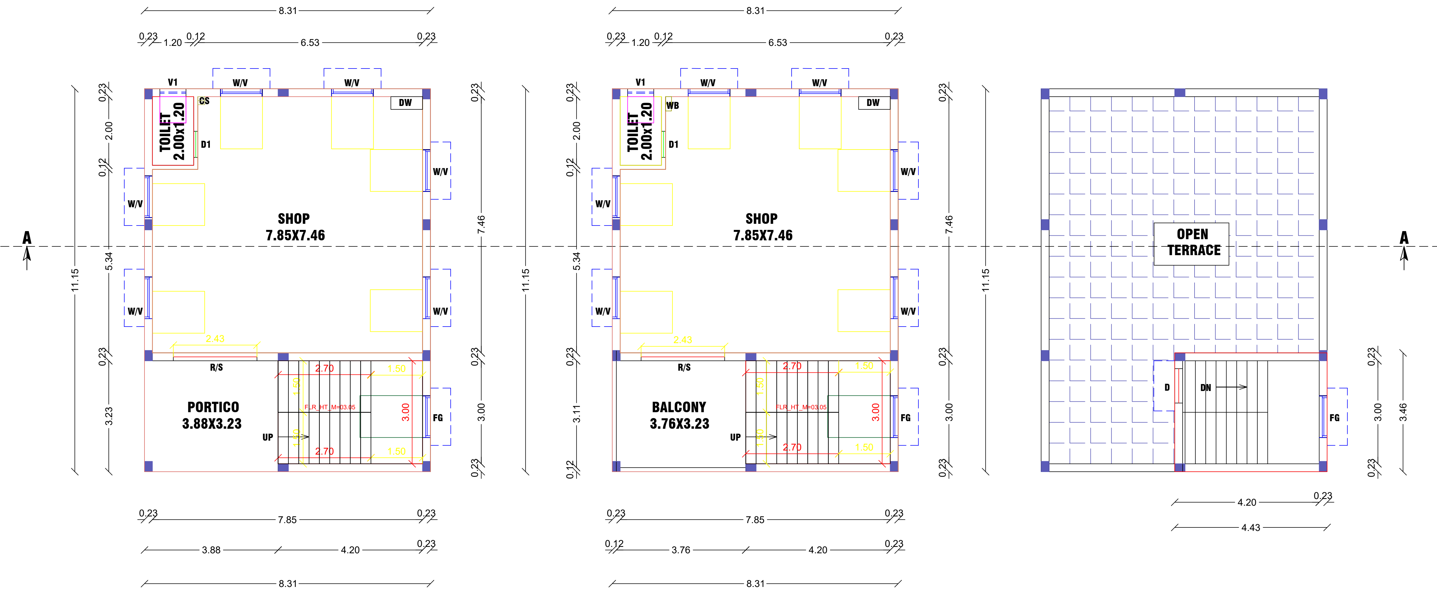
FLOOR-GROUND
