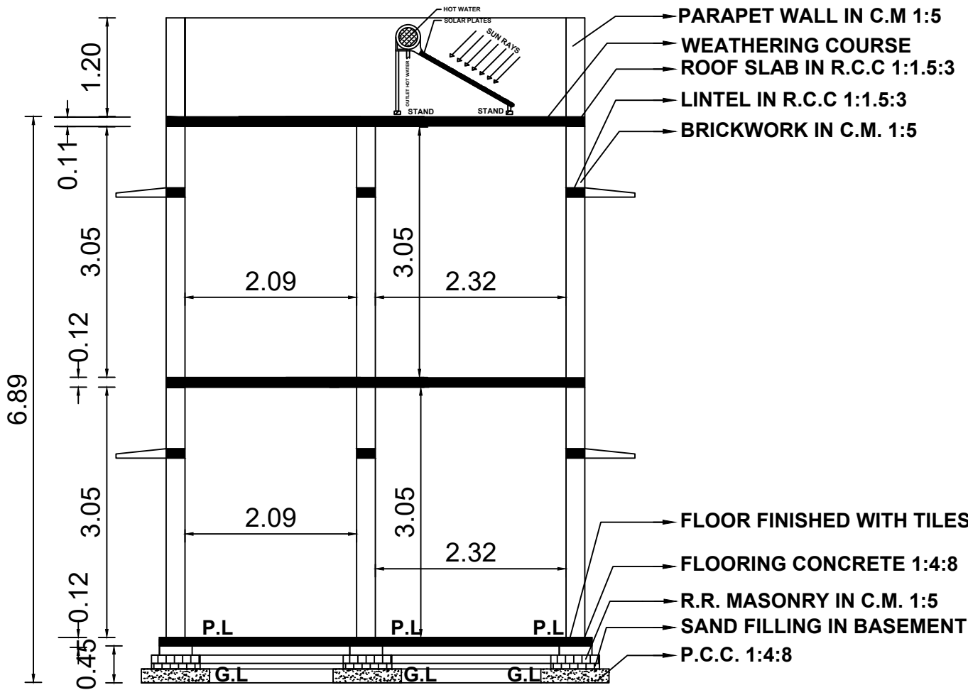
SECTION PLAN ON AA
