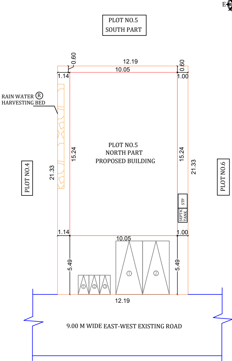
SITE PLAN
