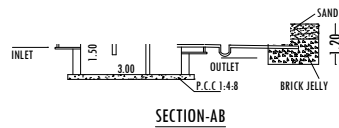
SECTION-AB
