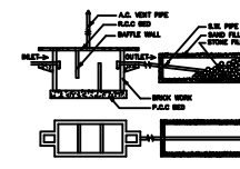
SEPTIC TANK DETAILS
