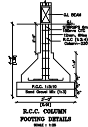
R.C.C. COLUMN FOOTING DETAILS
