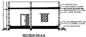
SECTION ON A-A
