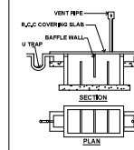
SEPTIC TANK DETAILS
