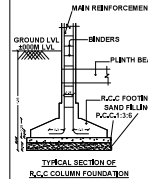
TYPICAL SECTION OF R.C.C. COLUMN FOUNDATION
