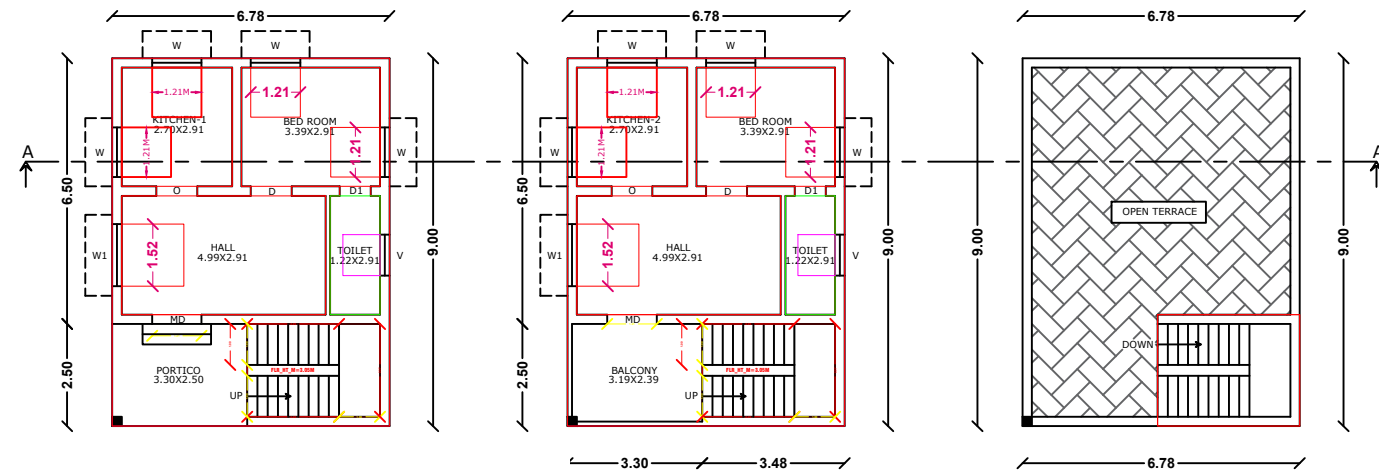
FLOOR - FIRST PRO. FIRST FLOOR PLAN
