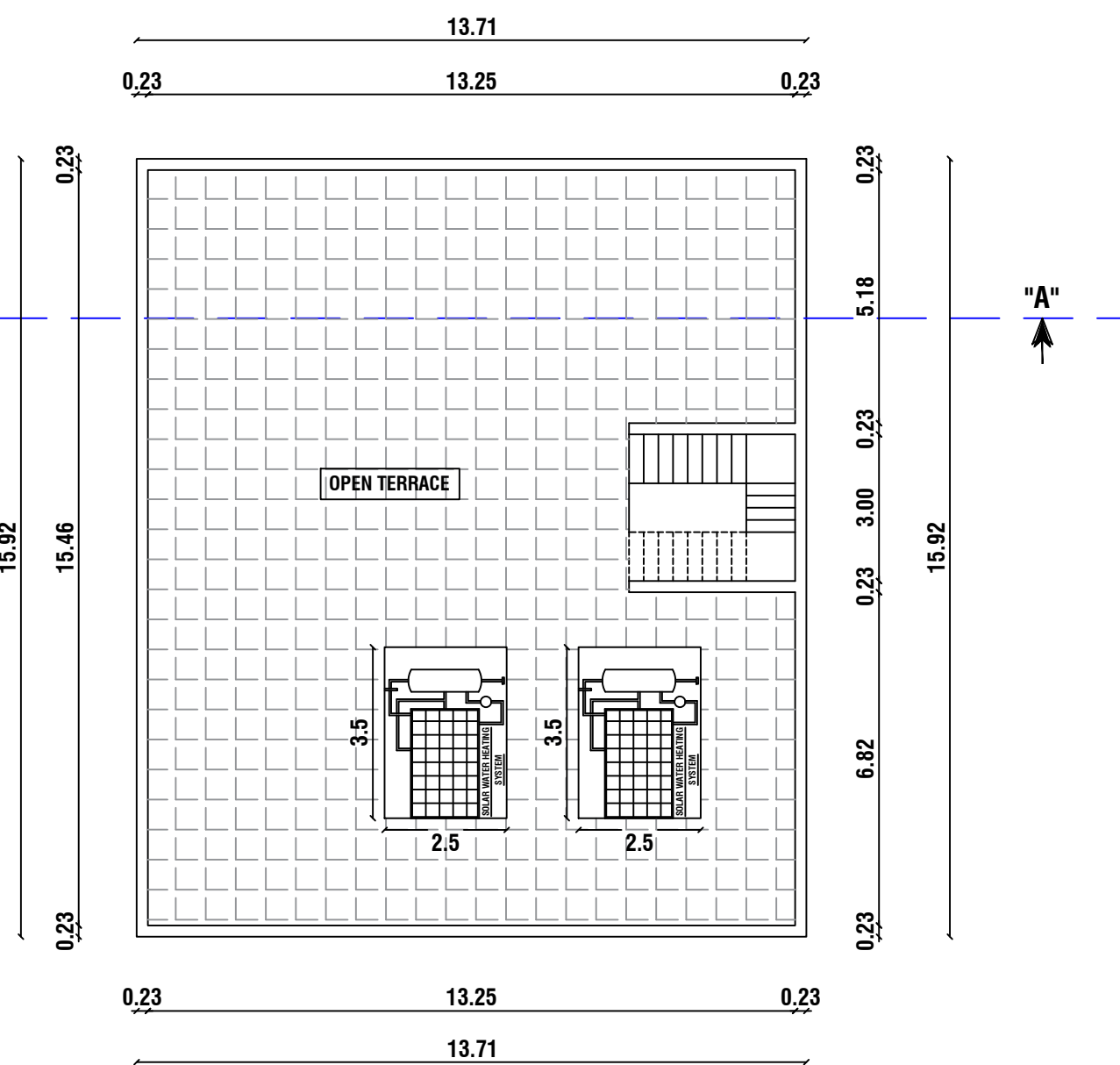
FLOOR - TERRACE PRO. TERRACE FLOOR PLAN
