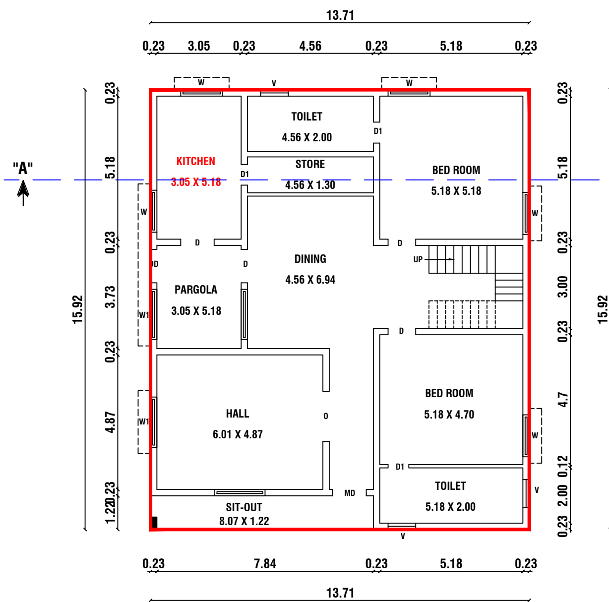
FLOOR - GROUND PRO. GROUND FLOOR PLAN
