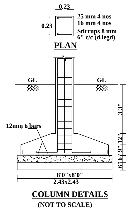
COLUMN DETAILS (NOT TO SCALE)
