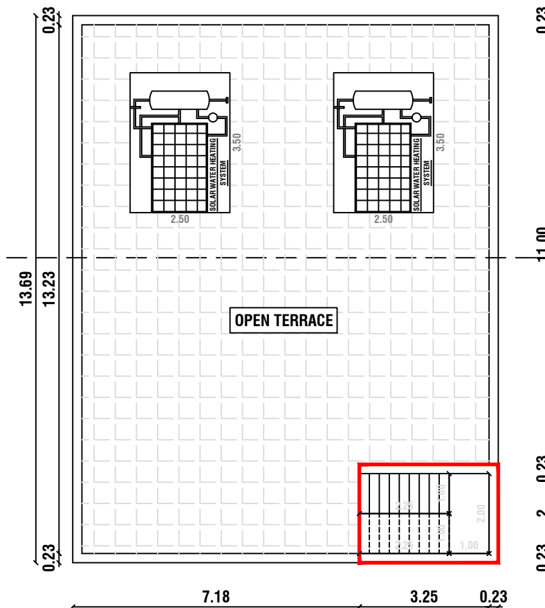
FLOOR - TERRACE PRO. TERRACE FLOOR PLAN
