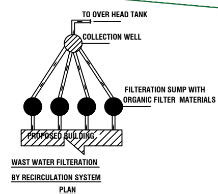
WAST WATER FILTRATION BY RECIRCULATION SYSTEM
