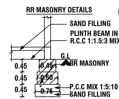
RR MASONRY DETAILS
