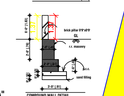
COMPOUND WALL DETAIL scale: 1/4" = 1'-0"
