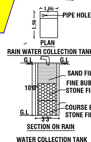
RAIN WATER COLLECTION TANK
