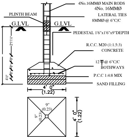
FOUNDATION DETAIL
