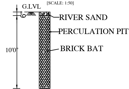
PERCOLATION PIT
