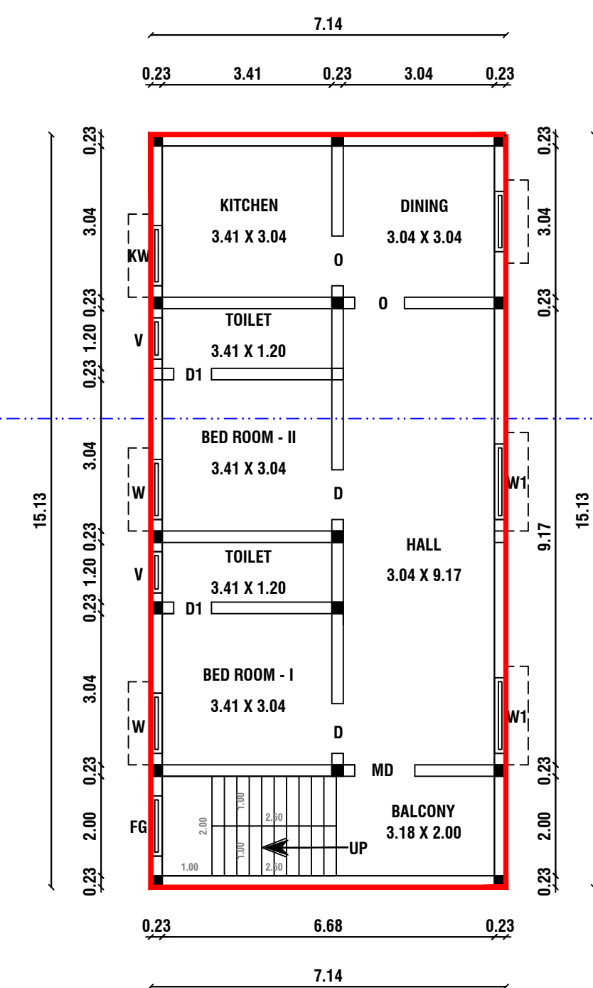
FLOOR - FIRST PRO.FIRST FLOOR PLAN
