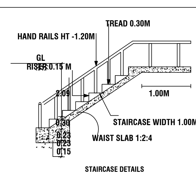
STAIRCASE DETAILS
