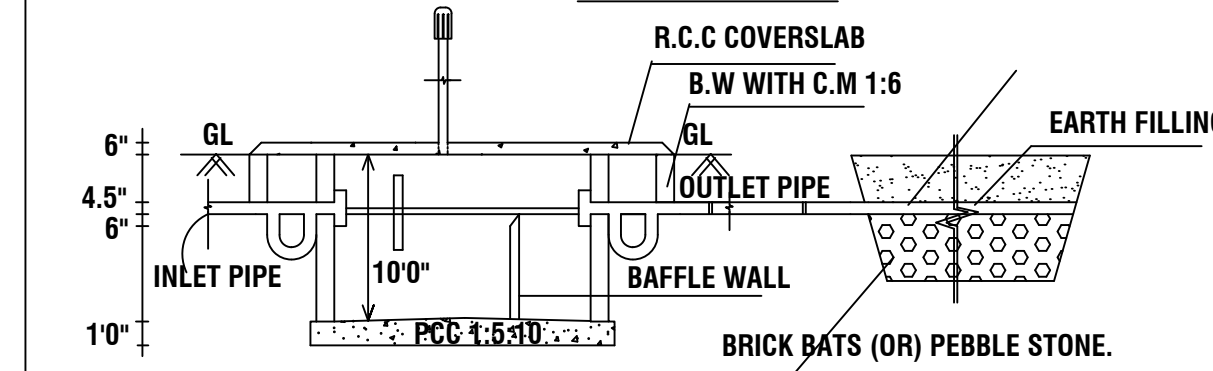
SEPTIC TANK DETAILS
