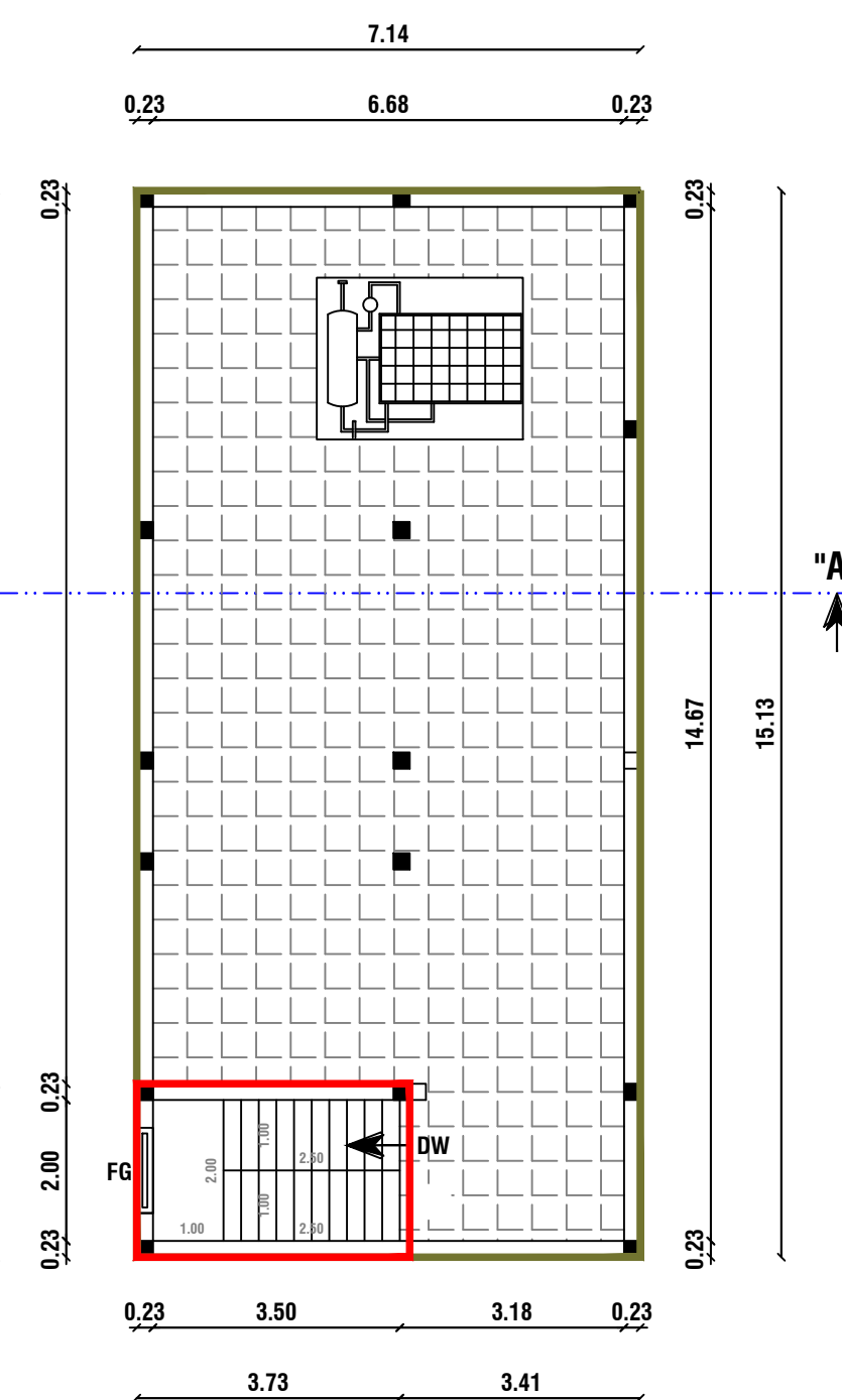
FLOOR - TERRACE PRO.TERRACE FLOOR PLAN
