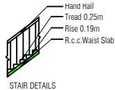
STAIR DETAILS
