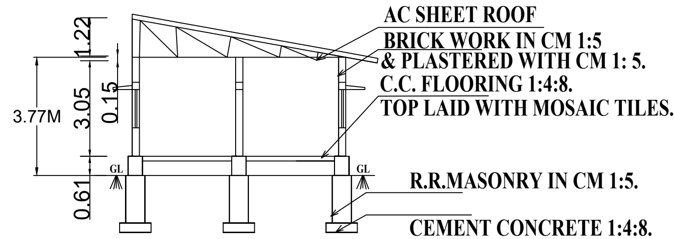
SECTION "A-B"
