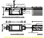
DETAILS OF SEPTIC TANK & DISPERSE
