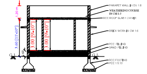
SECTION - "SR"
