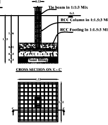
CROSS SECTION ON C-C
