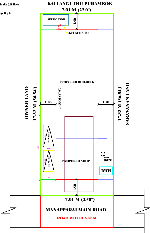
SITE PLAN
