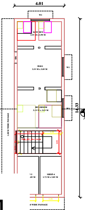
FLOOR PLAN
