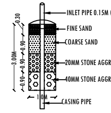
DETAILS OF RAIN WATER HARVESTING STRUCTURES
