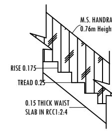
STAIRCASE DETAILS
