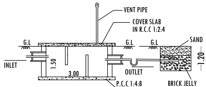
SECTION-AB
