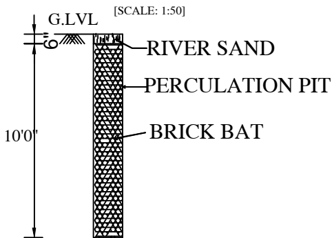
PERCOLATION PIT
