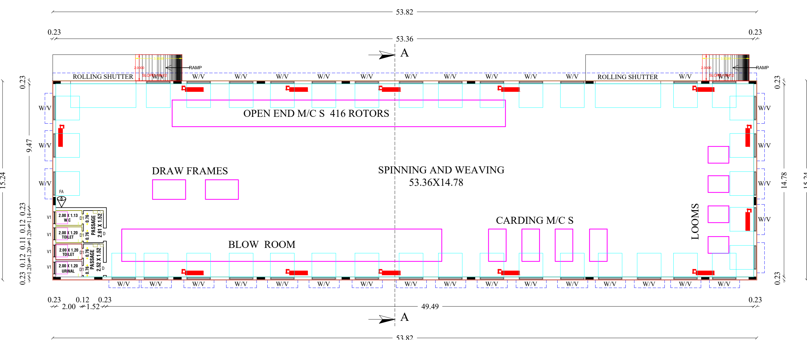
FLOOR-GROUND PRO.GROUND FLOOR PLAN (SPINNING AND WEAVING)
