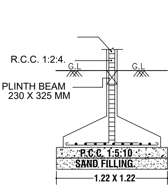
FOUNDATION DETAIL (NOT TO SCALE)
