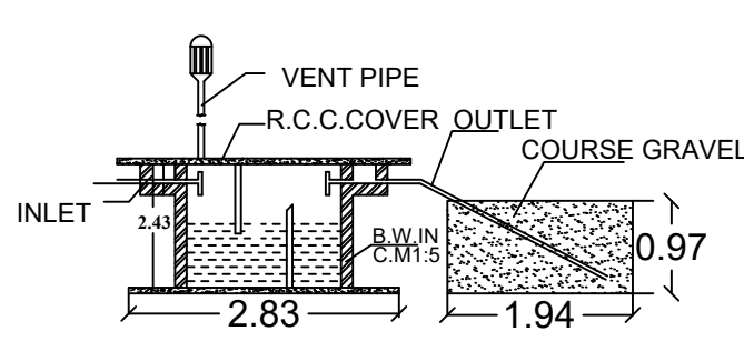
SEPTIC TANK & D-TRENCH DETAILS NOT TO SCALE
