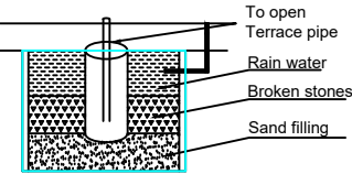
RAIN WATER COLLECTION CHAMBER
