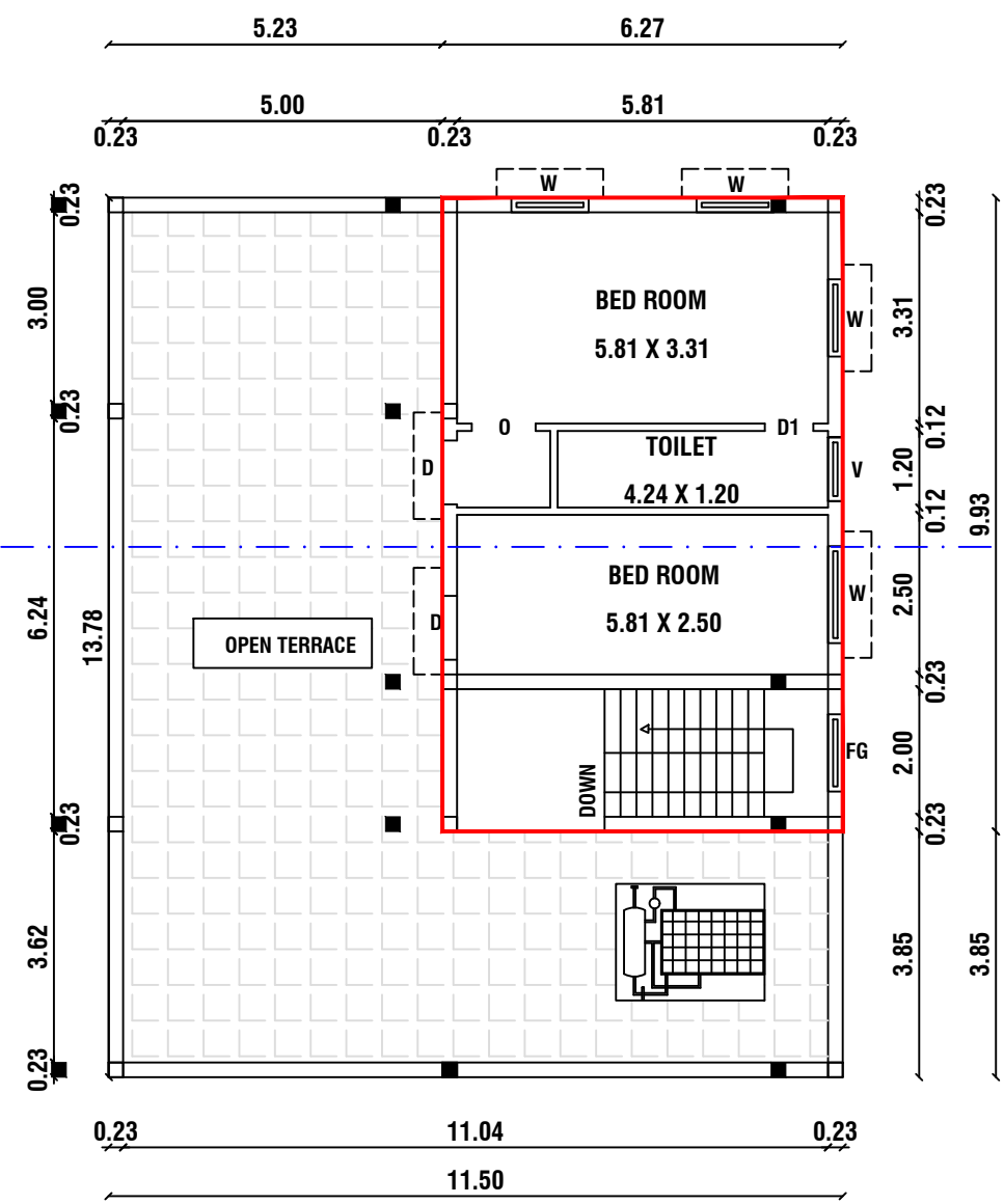
PRO. SECOND AND TERRACE FLOOR PLAN
