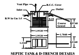
SEPTIC TANK & D-TRENCH DETAILS
