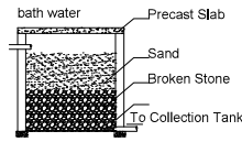
Section of Filter Unit
