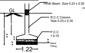
FOUNDATION DETAILS
