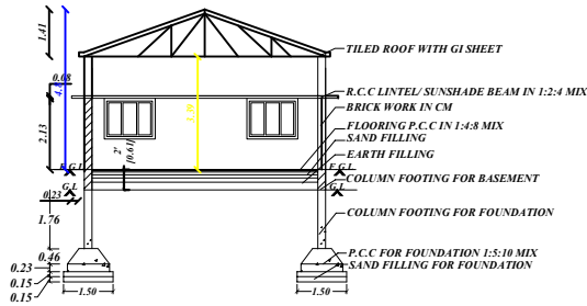
SECTION ON-AA
