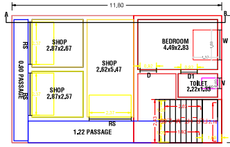
PRO FIRST FLOOR PLAN
