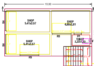
PRO GROUND FLOOR PLAN
