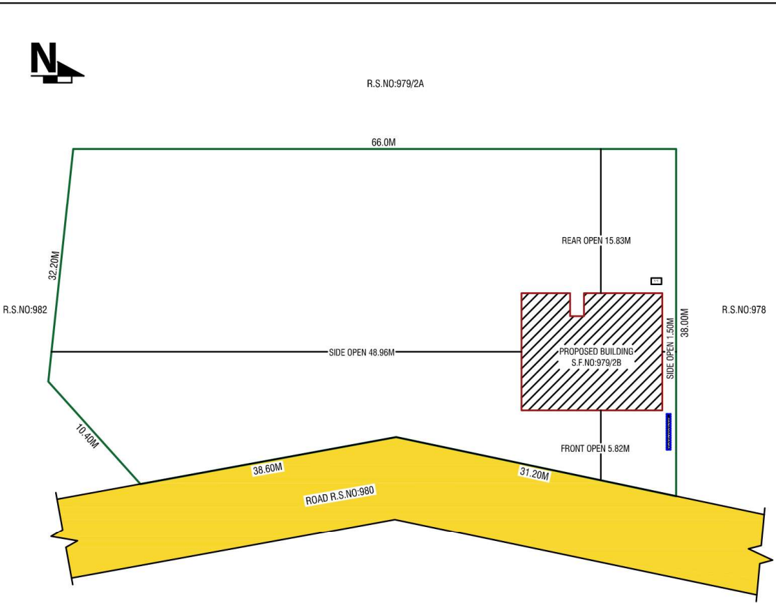
SITE PLAN
