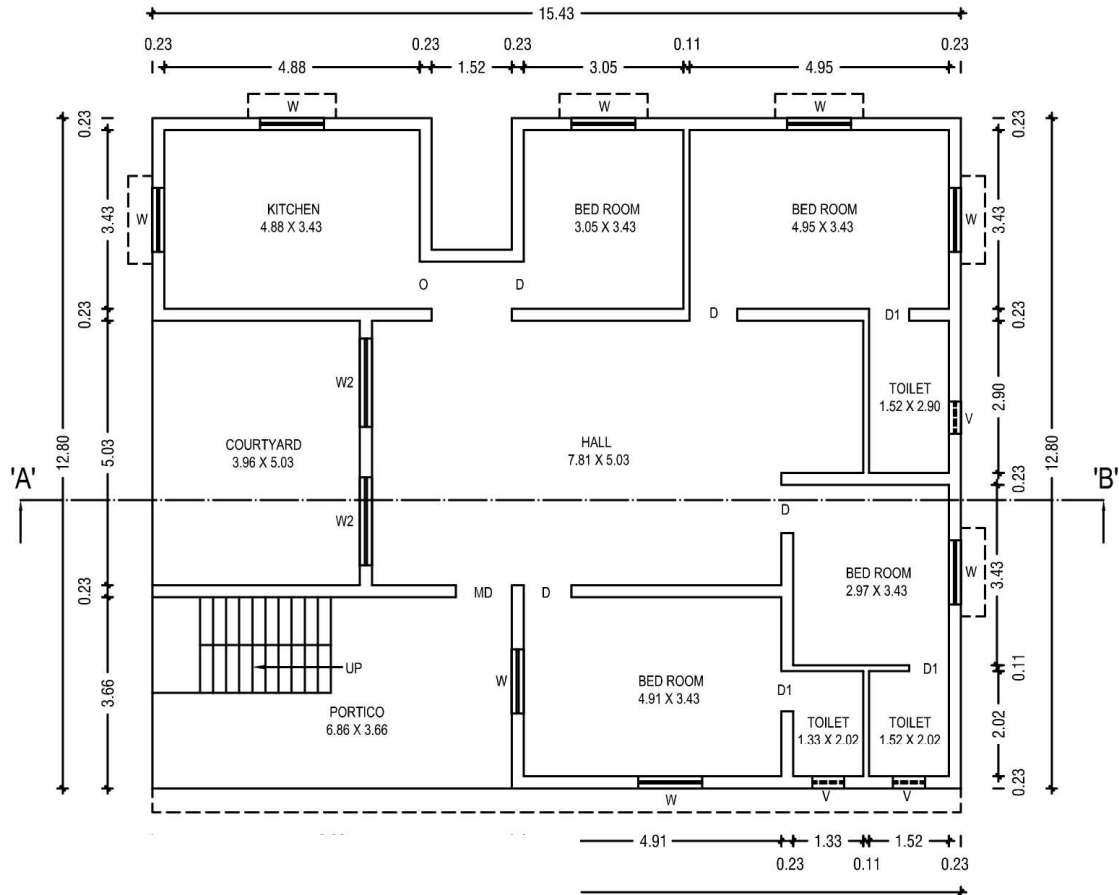
FLOOR PLAN
