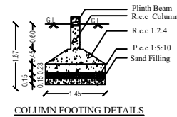
COLUMN FOOTING DETAILS
