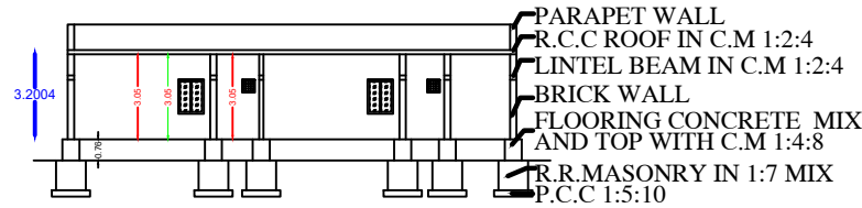
SECTION ON "A-A"
