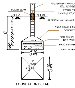
FOUNDATION DETAIL
