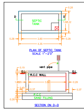
SECTION ON D-D
