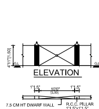
COMPOUND WALL PLAN
